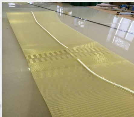
550 WT10 5820 longitudinal joint + V-Guide (confection & loading)
